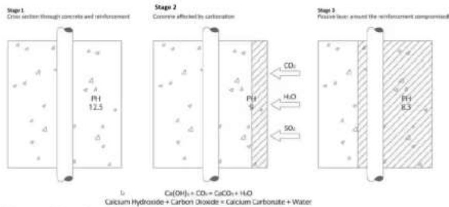
Figure 1: The carbonation of concrete
